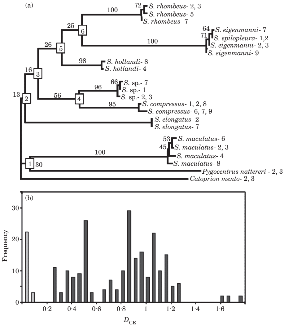
FIG. 2. (a) Neighbour-joining phenogram based on Cavalli-Sforza and Edwards's (1967) chord distance ( D_{CE} ) and rooted with Catoprion mento . Confidence values for nodes are percentages over 100 replicates. Nodes numbers referred to the allelic key to species in Appendix. Note that bootstrap proportions strongly support each species (see Table I) except for the differentiation of Serrasalmus eigenmanni ( S.eig ) and Serrasalmus spilopleura ( S.spi ). (b) Mistmatch distribution of pair-wise distances between populations (□) and species (■).
