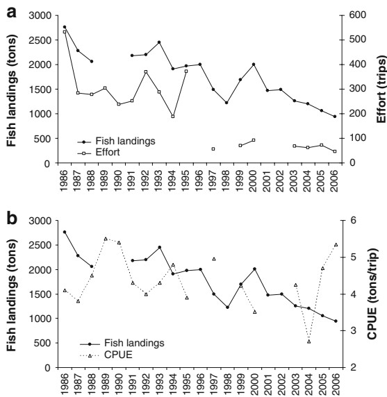
Fig. 14a, b Fish landings of the commercial fishery fleet of Iquitos and (a) effort (in number of trips) and (b) catch per unit effort (CPUE) during the period from 1986 to 2006
